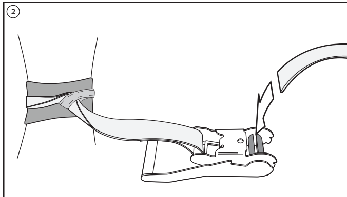
2 REPEAT WITH RATCHET END WHILE POSITIONING THE RATCHET UPSIDE DOWN. INSERT THE SLACKLINE THROUGH THE SLIT OF THE RATCHET DRUM.
