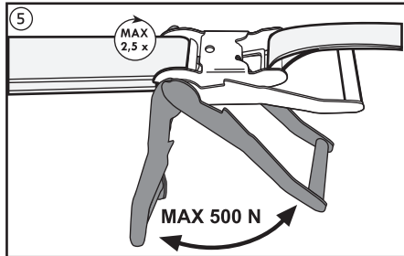
5 COIL UP THE LINE NOT MORE THAN 2,5 REVOLUTIONS. APPLY NO MORE THAN 500N (50KG/100LBS) ON THE LEVER.
