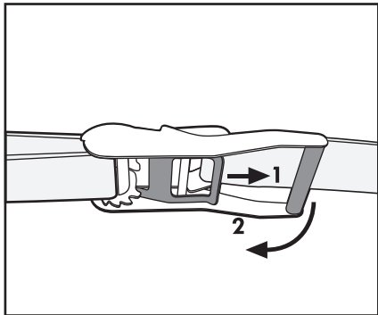
RELEASE THE SAFETY LEVER AND OPEN RATCHET LEVER
